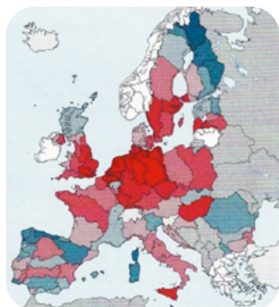
Fig 1. Ecological status of water/potential bodies in Europe's River Basin Districts in second River basin Management Plans.
